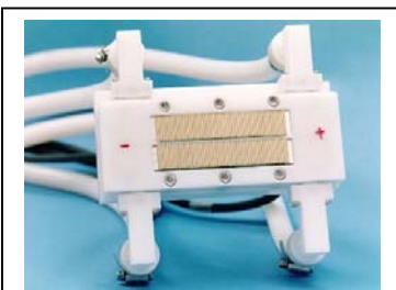
Figure 10: Laser diode array
